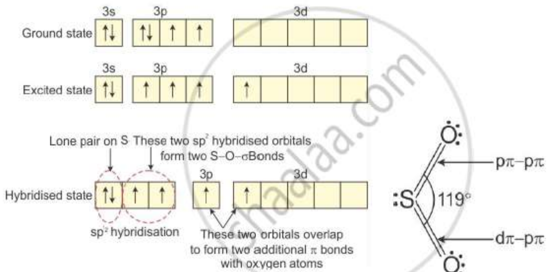
Hybridisation of S in \text{SO}_2 molecule Bonding in \text{SO}_2 molecule
